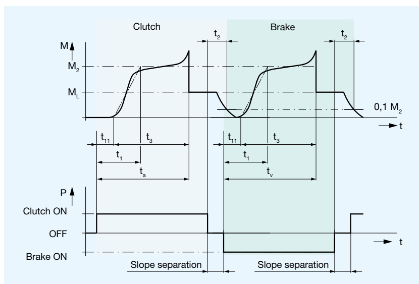
Diagram 3: Torque-Time Diagram
