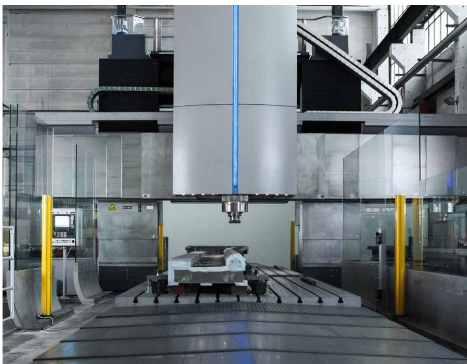
WaldrichSieggen portal milling machine ProfiMill with planetary gearbox PSD30
