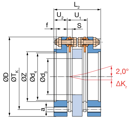
Fig. 56: Type 951.661
