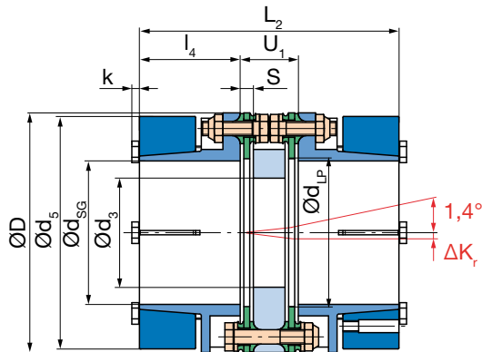
Fig. 26: Type 953.991
