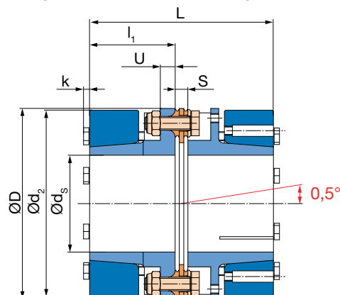
Fig. 62: Type 950.220
