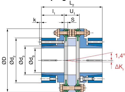
Fig. 23: Type 953.231
