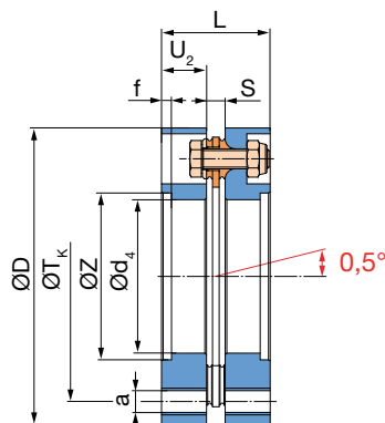
Fig. 68: Type 950.660
