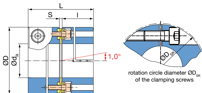
Fig. 1: Type 950.440
