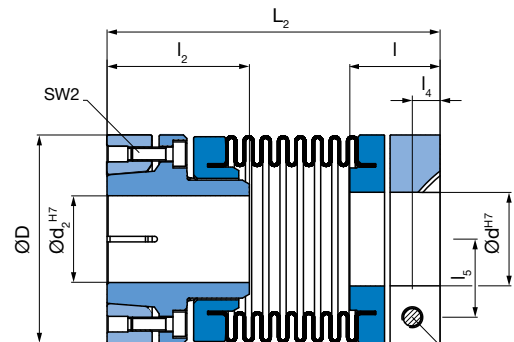
Type 933.535.1 without keyway Type 933.567.1 with keyway SW1
