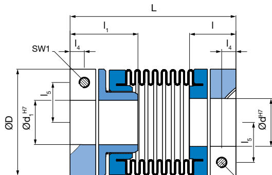
Type 933.533.1 without keyway Type 933.566.1 with keyway SW1
