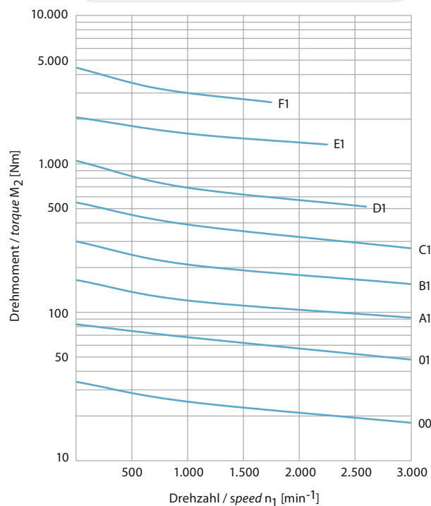
i = n_1 : n_2 = 4:1 (Standard)
