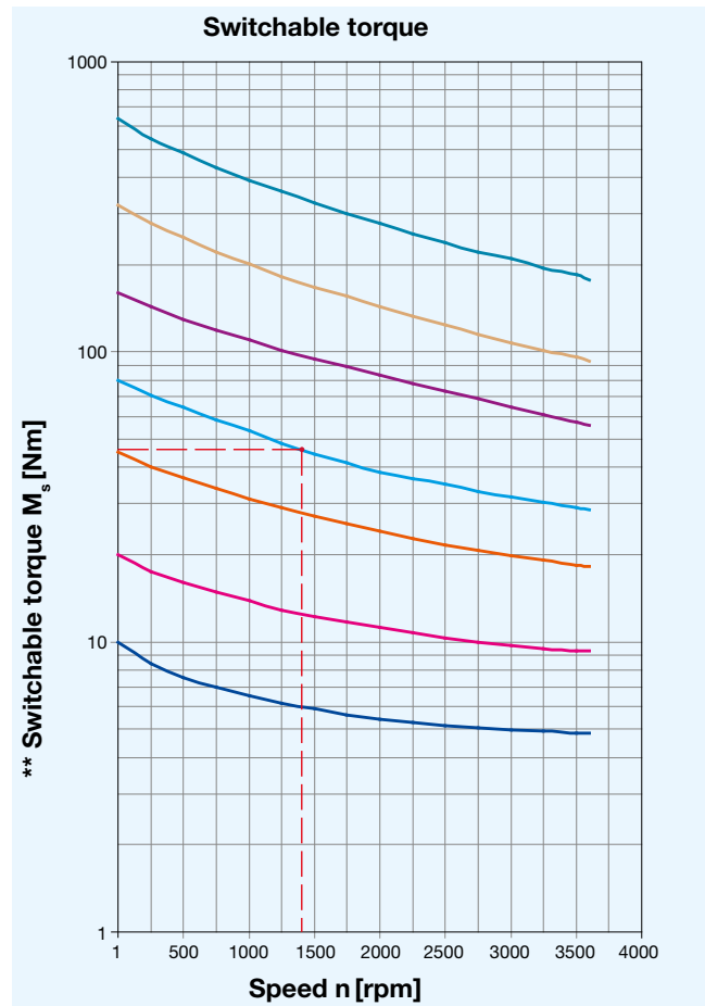
Diagram 1 (not valid for Type 500.30_)
