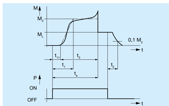
Diagram 3: Torque-Time Diagram
