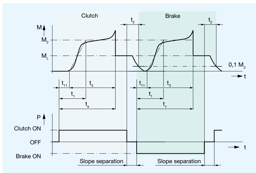
Diagram 3: Torque-Time Diagram
