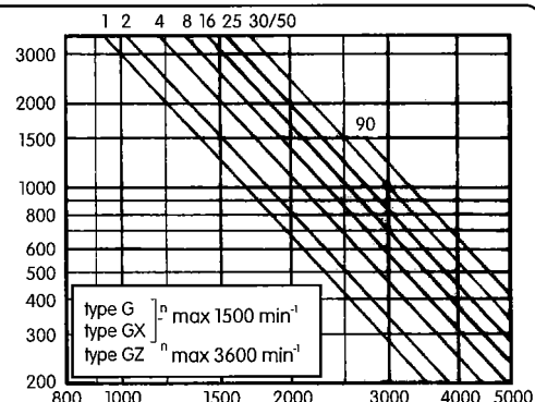
RPM - length - diagram:
