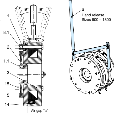
Fig. 3 (Single circuit brake)
