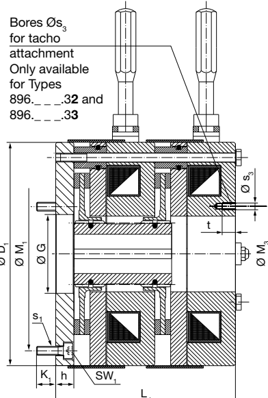
Type 896.005.33 (Dual circuit brake)
