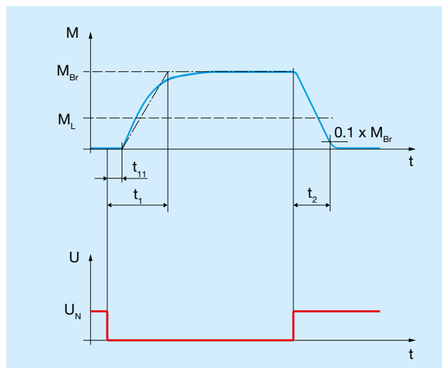
Diagram 4: Torque-Time Diagram
