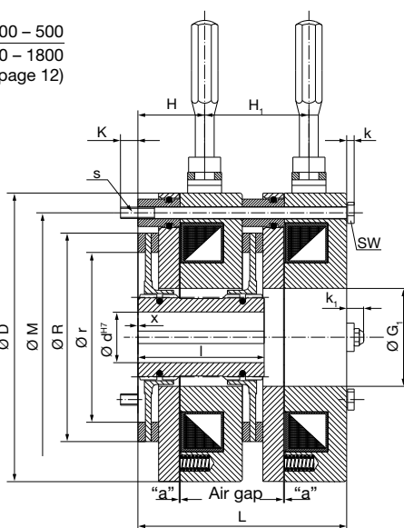
Type 896.001.30 (Dual circuit brake)
