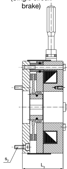
Type 896.105.33 (Single circuit brake)
