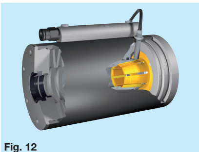
Design with increased corrosion protection
