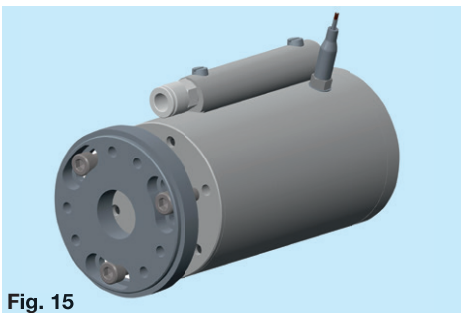
Positioning flange
